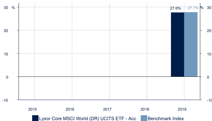
Annual performance of Lyxor Core MSCI World (DR) UCITS ETF - Acc (in %)
